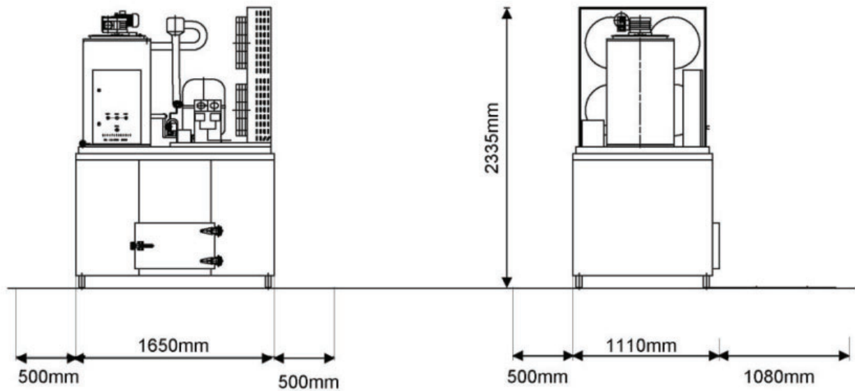
FIM-100 external dims. and clear working space required
